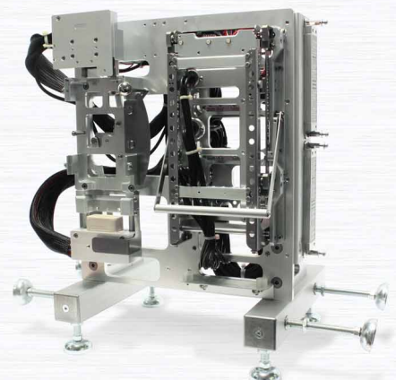
Control unit test bench for temperature cycle testing
